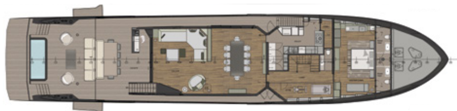
MAIN DECK
