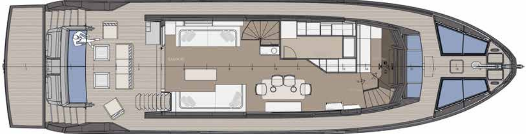
MAIN DECK Lounge Version
